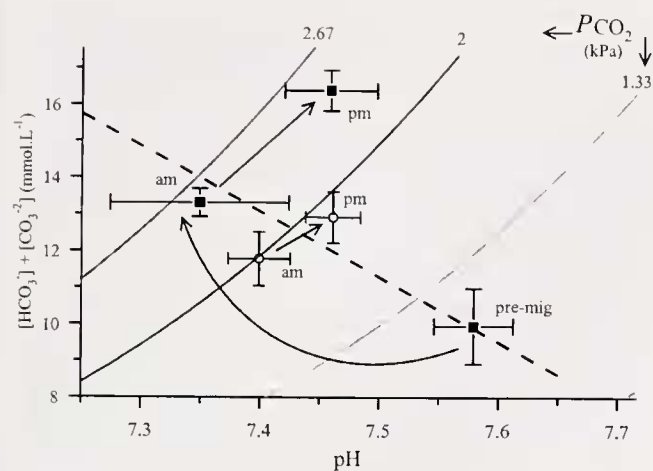
Figure 7. The pH/Bicarbonate relationship for Gecarcioidea natalis during two migration seasons, (■) 1993 and (○) 1995. The pre-migratory values in 1993 were assumed to be applicable to the 1995 season. The P_{CO_2} isopleths were constructed using the Henderson-Hasselbalch equation using \alpha_{CO_2} = 0.03962 and pK = 6.1 . The non-bicarbonate buffer line was adopted from Adamczewska and Morris (1994a).
